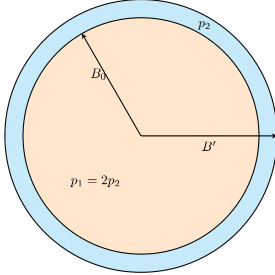
Figure 1: Double Sphere Distribution
